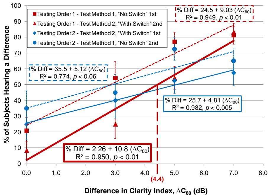
Figure 14: C80 JND results separated by the four combinations of testing order & test method.
