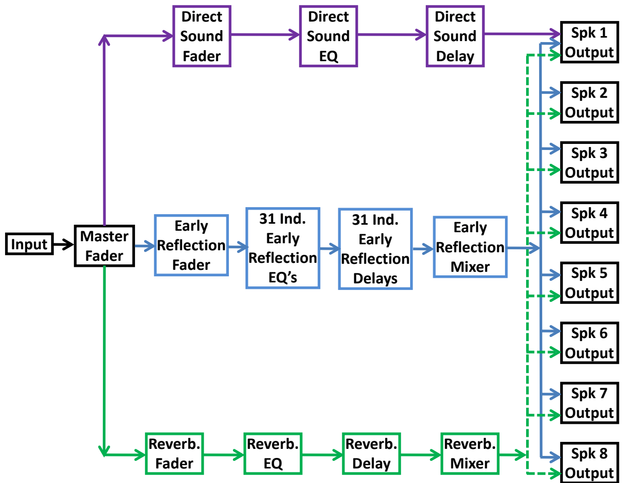
Figure 4: Overview of room impulse response signal generation for simulated sound fields.
