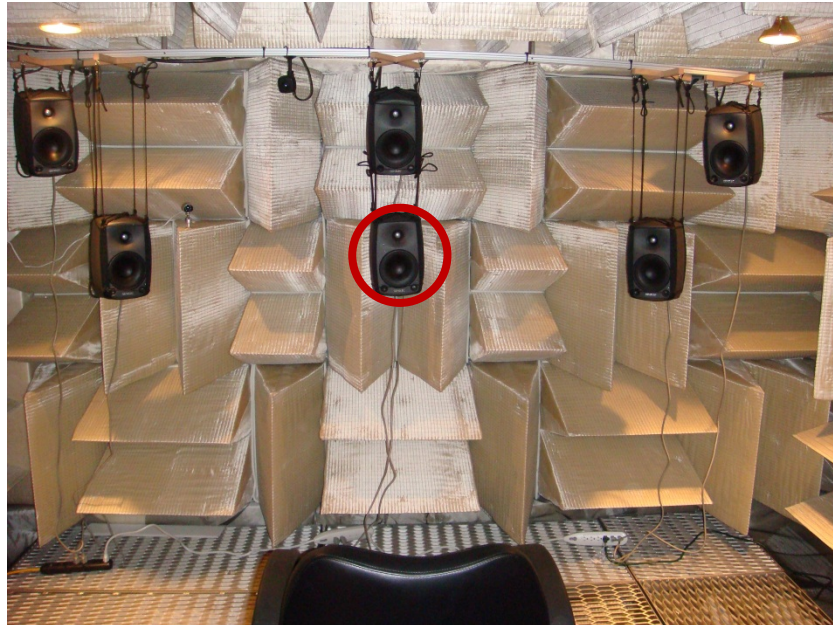
Figure 2: Six front loudspeakers as viewed from behind the listener's position.
