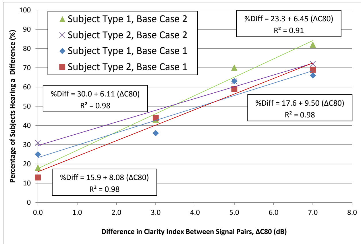
Figure 12: C80 JND results separated by the four combinations of subject type & base case.
