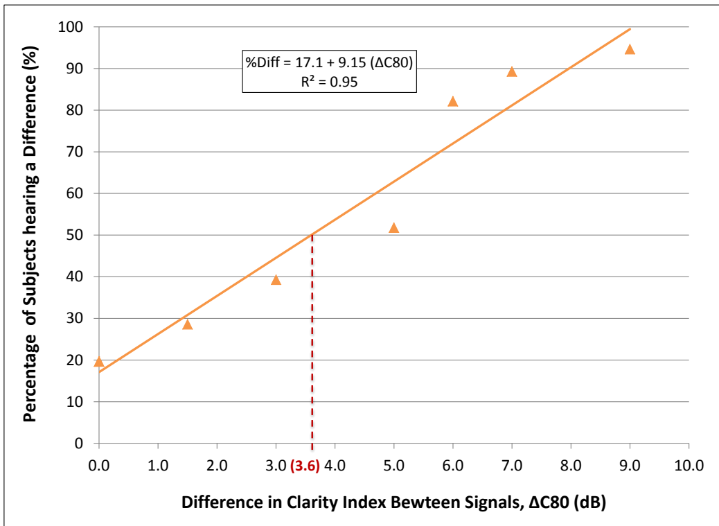
Figure 7: C80 JND Results for Base Case 2, C80 = 0.0 dB at 1 kHz and T30 = 1.6 s
