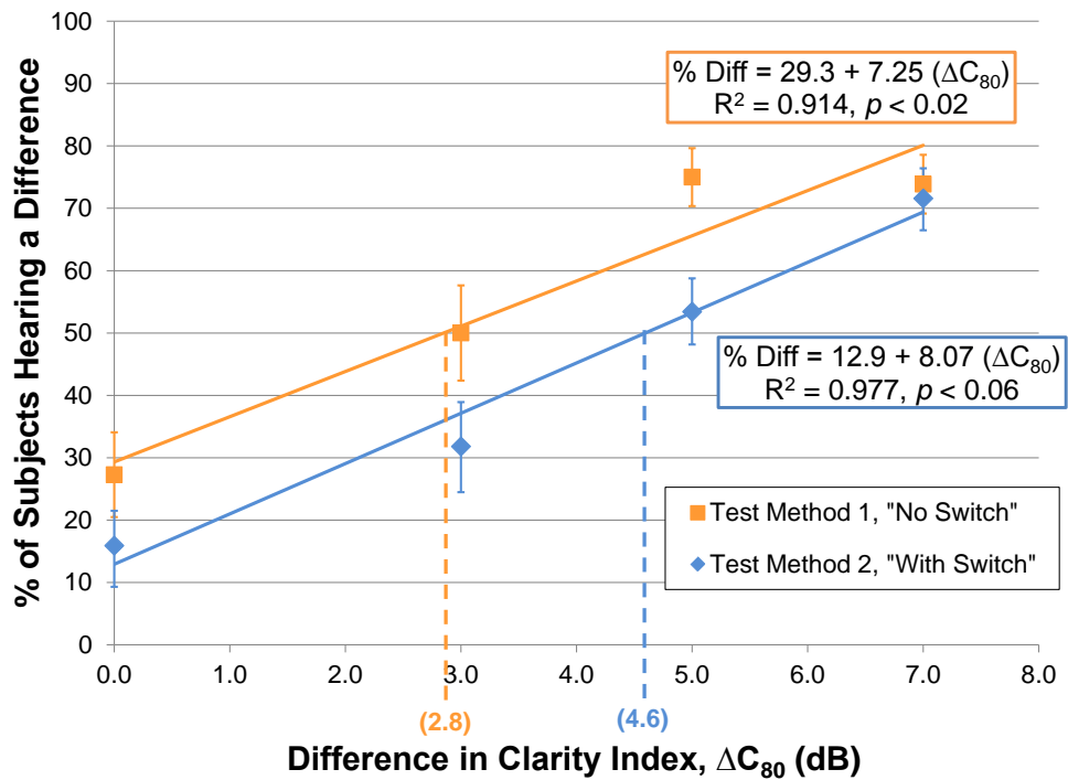
Figure 13: C80 JND results separated by test method.
