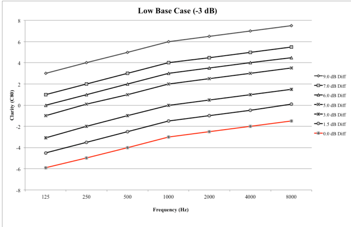
Figure 3: Clarity Values for Base Case 1 with C80 @ 1kHz = -3 dB and T30 of 1.9 s
