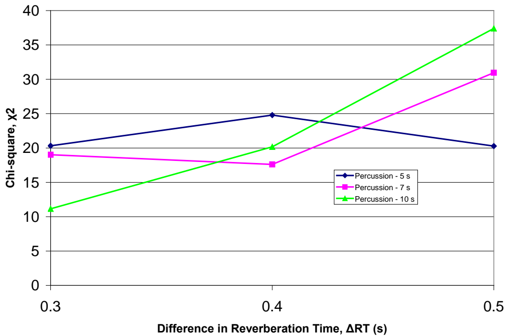
Figure 6: Plot of Chi-Square vs. \Delta RT for Percussion Motif at Varying Lengths
