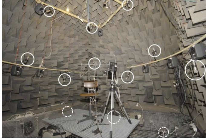
Figure 1: Dodecahedron Microphone placement
