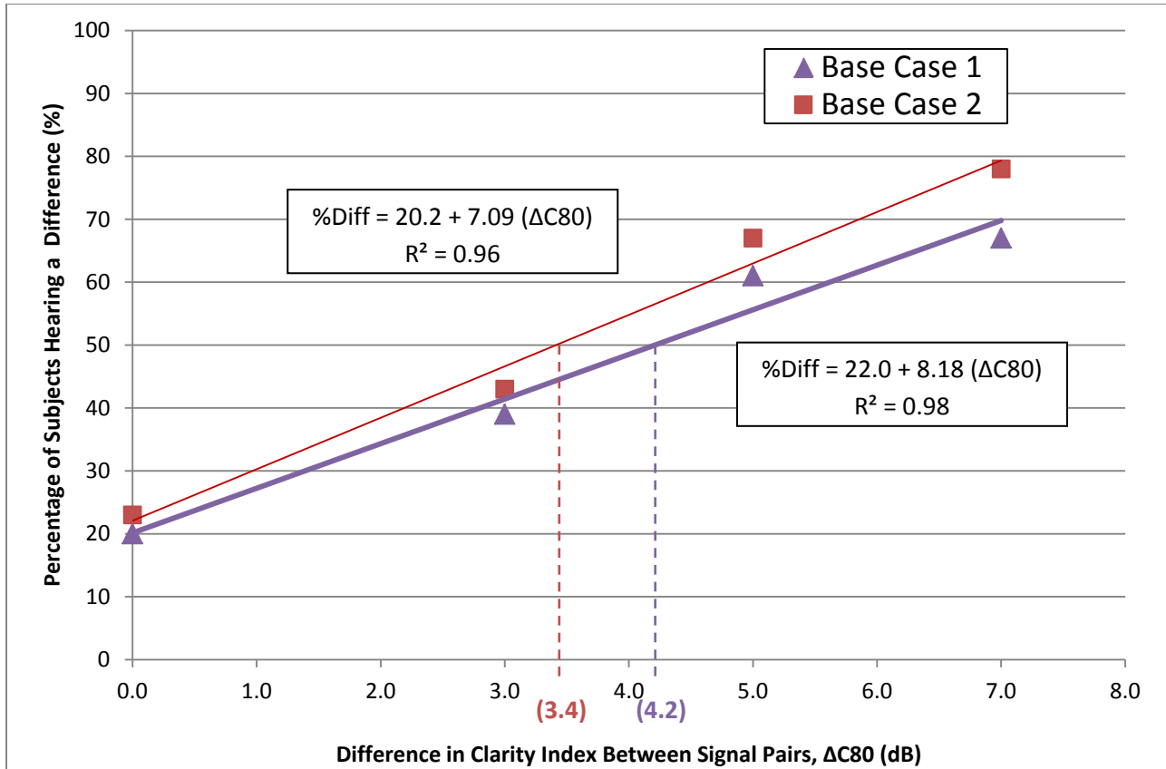
Figure 8: C80 JND results separated by base case.
