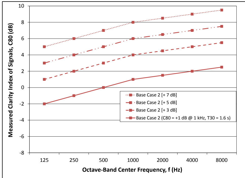
Figure 6: Measured clarity index values (C80) for 125 – 8000 Hz center octave bands for Base Case 2.
