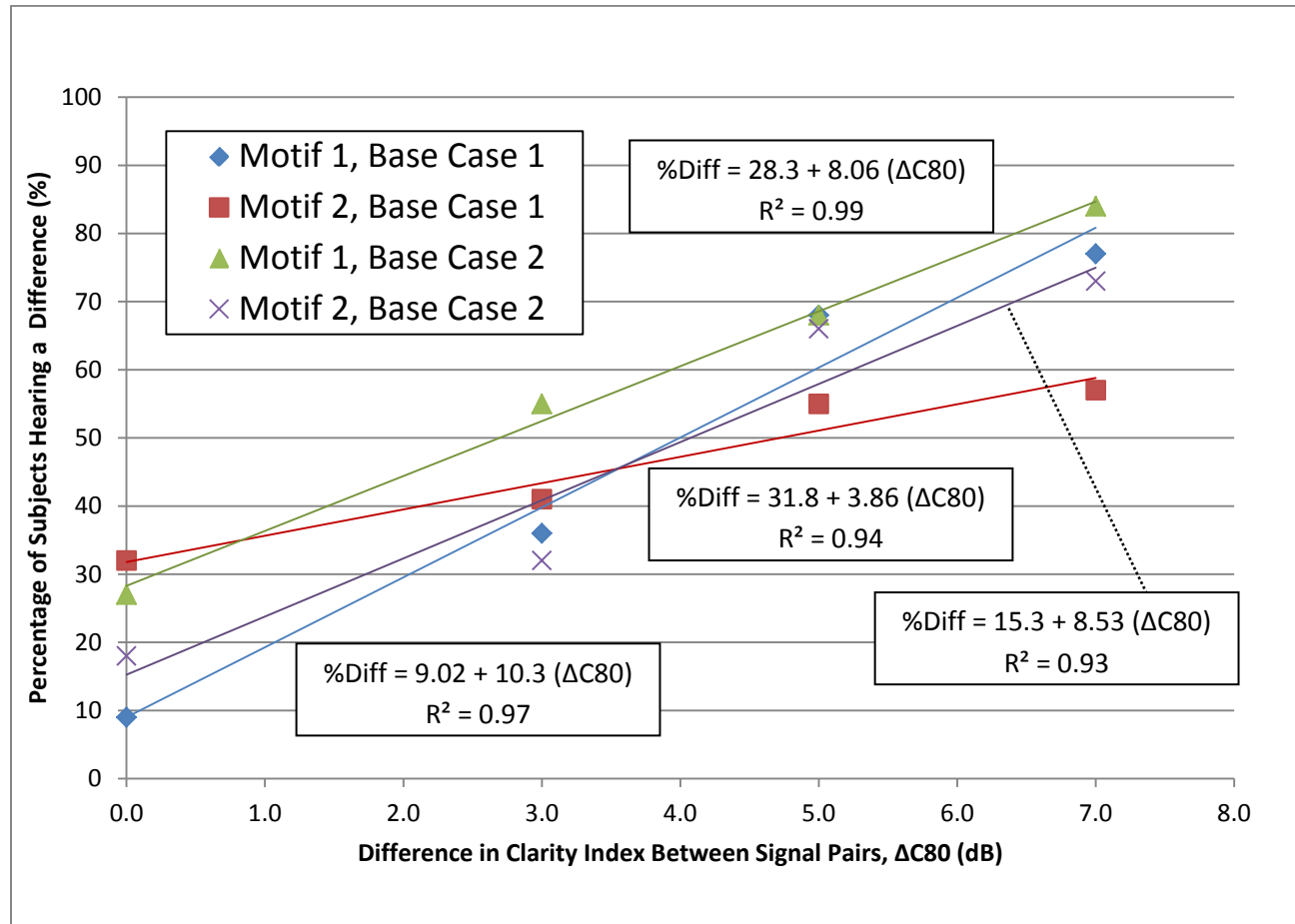
Figure 10: C80 JND results separated by the four combinations of motif & base case.
