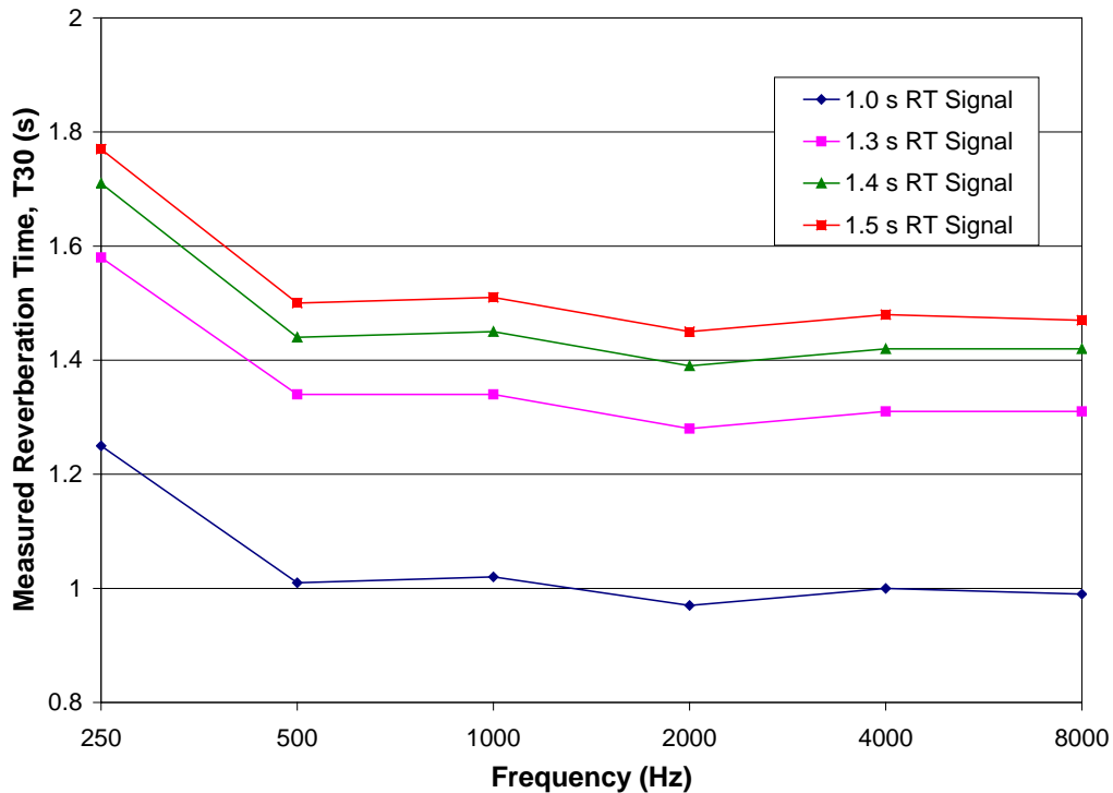
Figure 1: Measured Reverberation Time (T30) vs. Frequency
