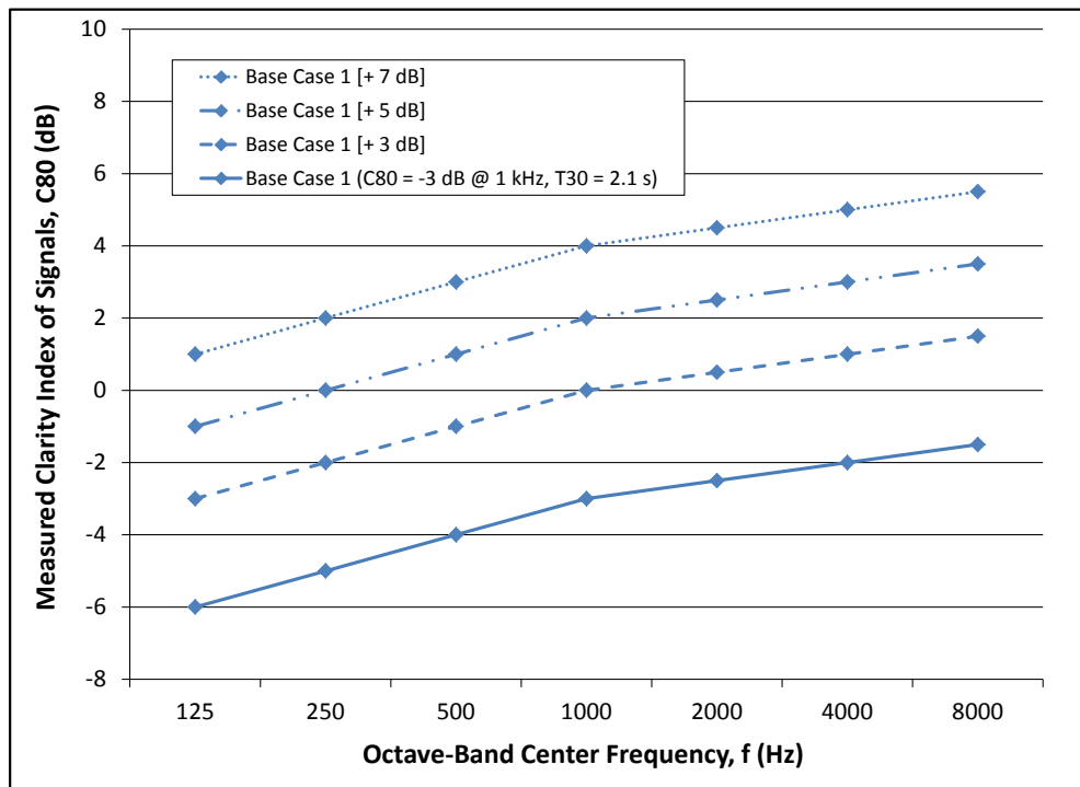
Figure 5: Measured clarity index values (C80) for 125 – 8000 Hz center octave bands for Base Case 1.
