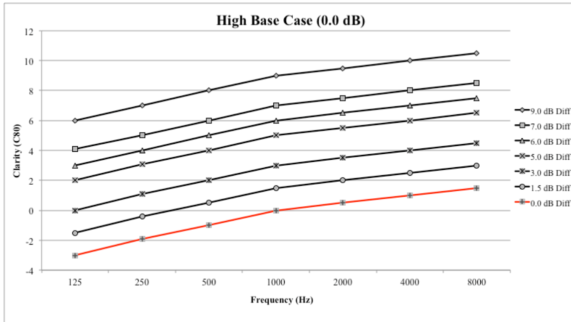
Figure 4: Clarity Values for Base Case 2 with C80 @ 1kHz = 0 dB and T30 of 1.6 s
